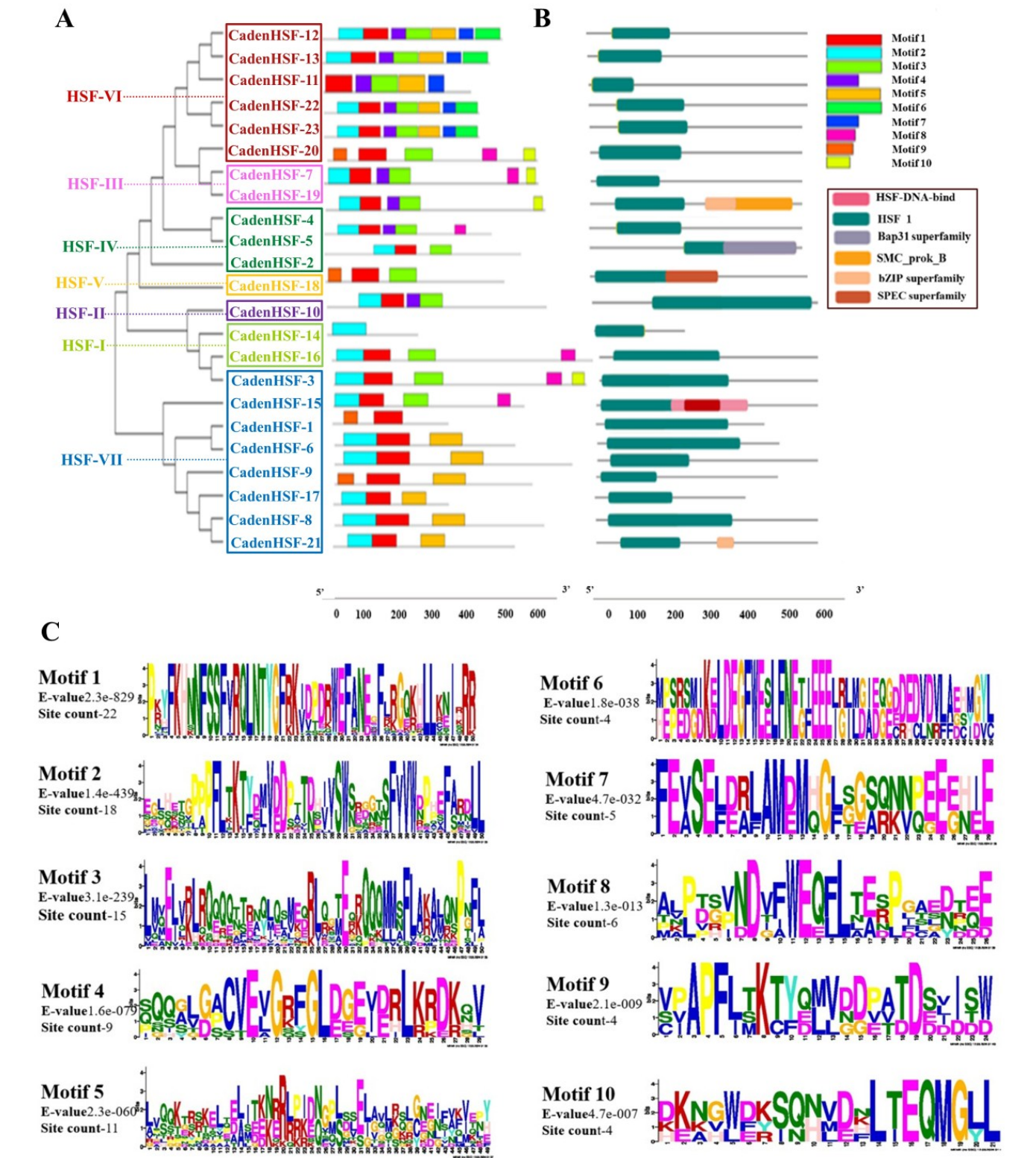
Figure 6. Functional domain and conserved motif analysis of the CadenHSFs gene family in Castanea dentata . (A) Distribution of 10 conserved motifs across 23 CadenHSFs proteins, organized according to phylogenetic relationships. Colored bars represent distinct motifs, highlighting the conservation and diversity within each subgroup. (B) Functional domain architecture of CadenHSFs proteins, where the color bar indicates conserved domains such as HSF. The presence of additional domains such as Bap31, SPEC, and bZIP indicates that some CadenHSFs proteins may have evolved specialized functions beyond canonical heat stress regulation. (C) Sequence logos of the 10 identified motifs, showing the conserved amino acid positions and sequence variability.
