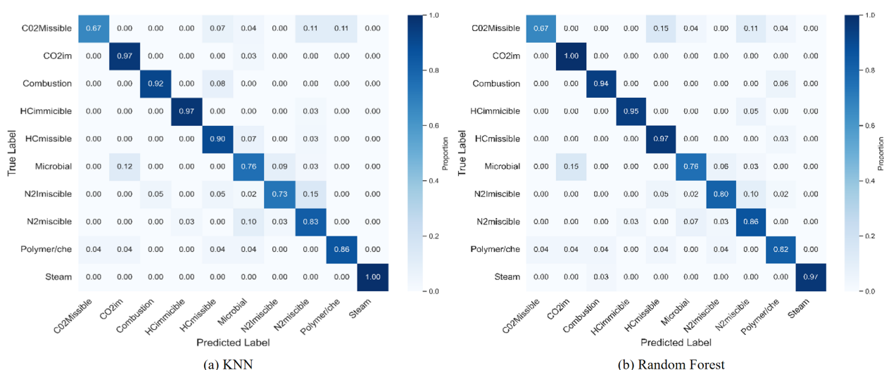
Figure 6. Confusion matrices for (a) KNN and (b) Random Forest.
