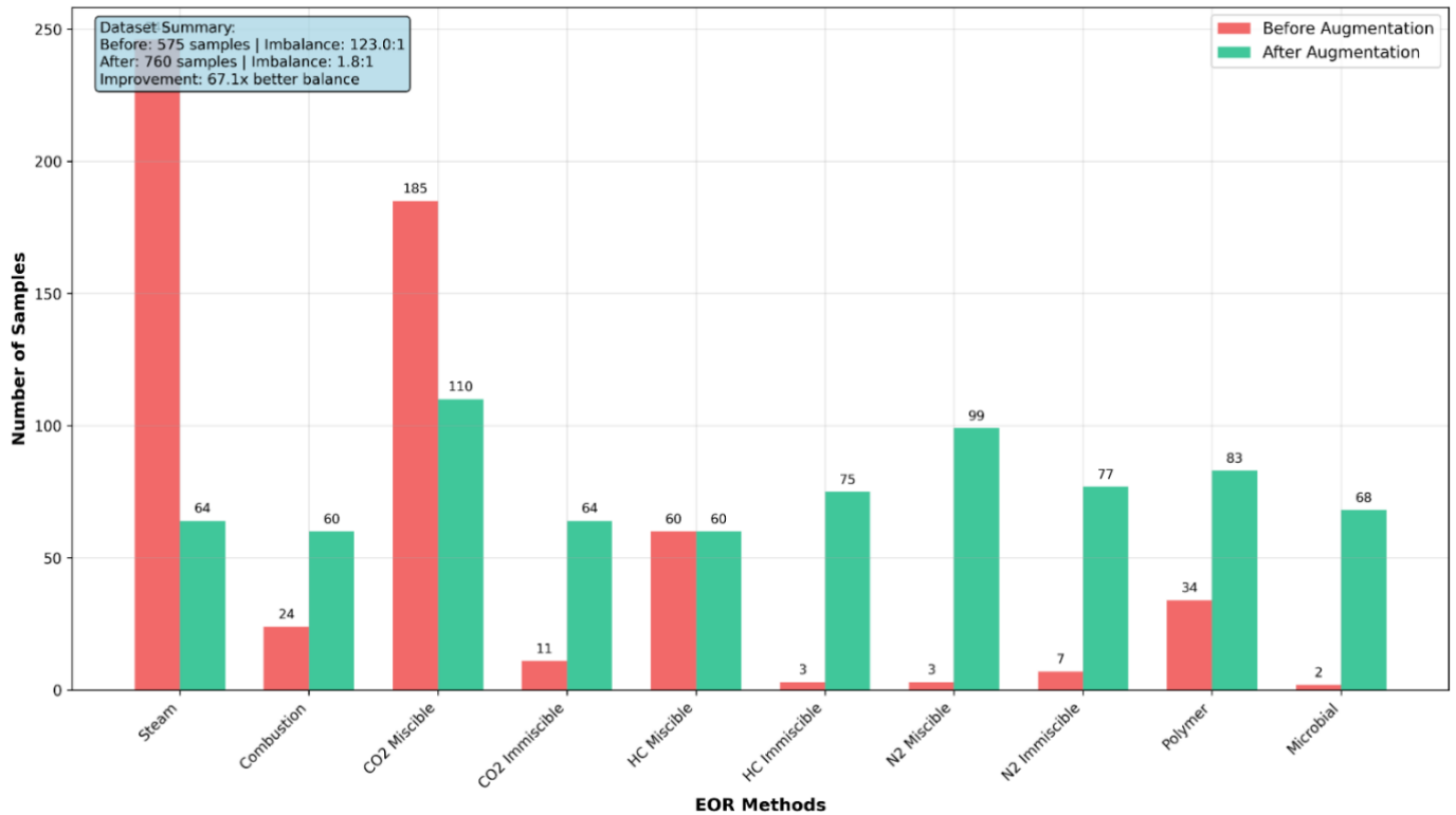
Figure 4. Sample Count Comparison Before and After Augmentation (Before: 575 samples with 123:1 imbalance; After: 760 samples with 1.8:1 imbalance).
