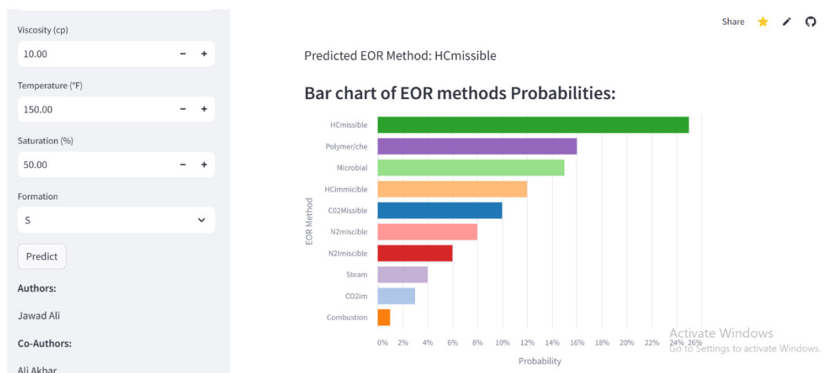
Figure 7. Streamlit application interface showing input sidebar (left) and output visualization with bar chart and probability table (right).
