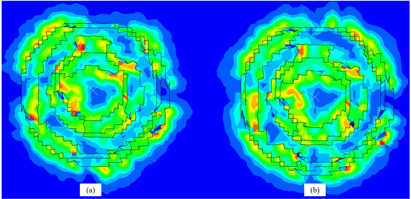
Figure 9. Stress distribution of hot dry rock breaking under coupling of impact load and confining pressure releasing (the static load is 50 kN, the impact load amplitude is from 10- 25 kN, impact load frequency is 6 Hz, confining pressure releasing \Delta p is 30, 60 MPa respectively, RPM is 120 r/min).
