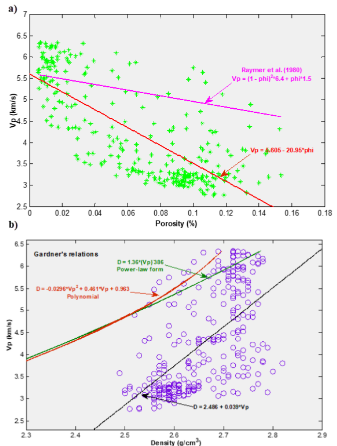
Figure 5. Cross-plots for Formation-1. (a) Velocity vs (b) Density.
