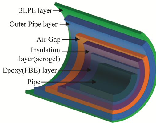
(b) Flowline
