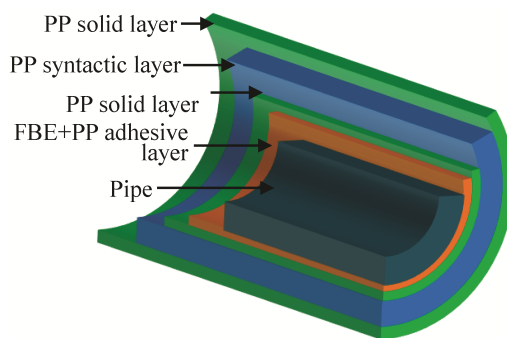
(c) Riser
