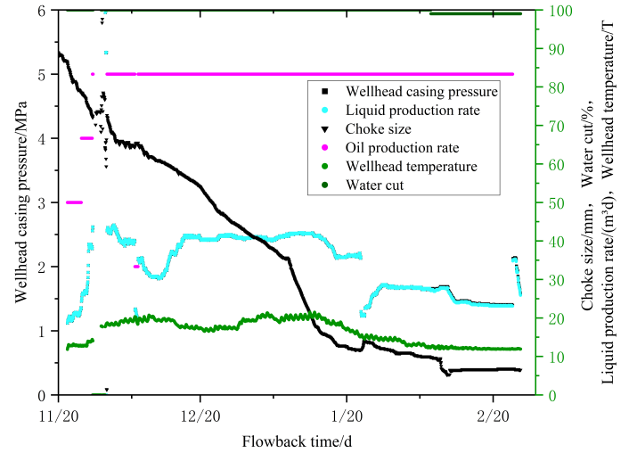
Figure 4. Historical flowback data of fracturing fluid for well H.
