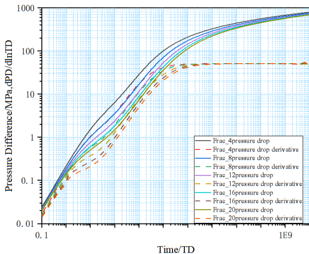
(c) k=0.5\text{md}
