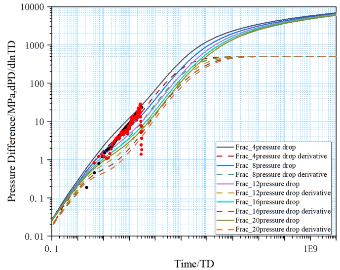
(a) Double Logarithmic Derivative Plot Fitted with Wellhead Casing Pressure
