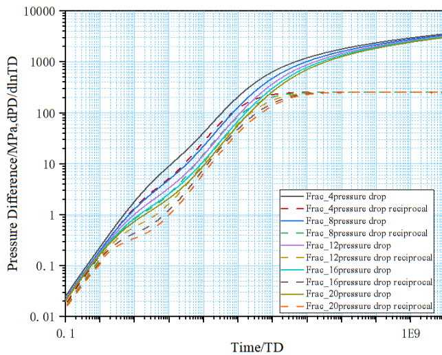
(b) k=0.1\text{md}
