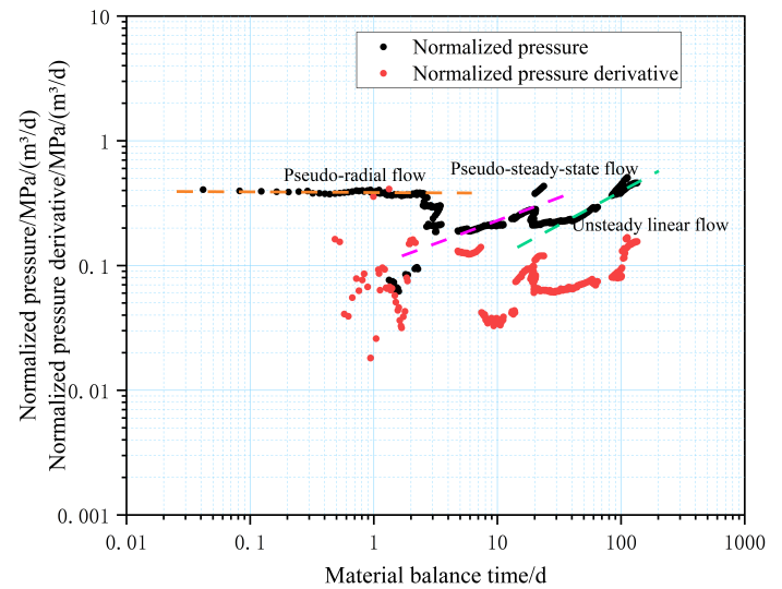
Figure 5. Double Logarithmic Derivative Plot of Production-Normalized Pressure vs. Material Balance Time.
