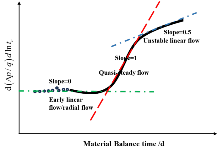
Figure 2. Characteristic flow stages during the flowback process.
