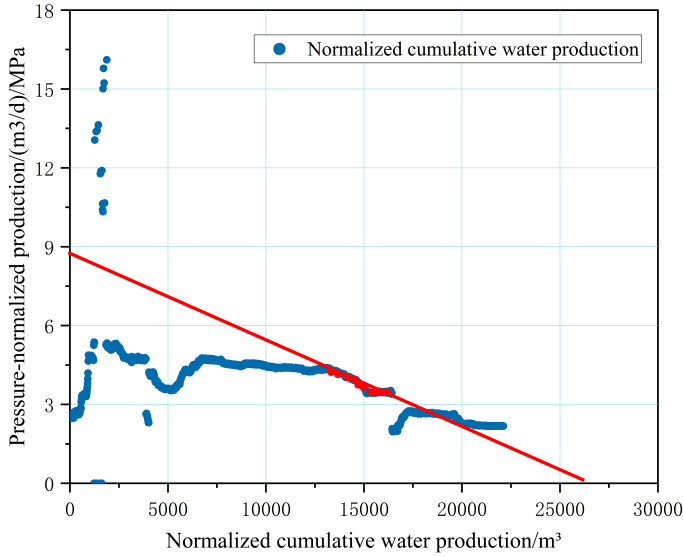
Figure 6. Pressure-Normalized Production vs. Normalized Cumulative Water Production Curve.
