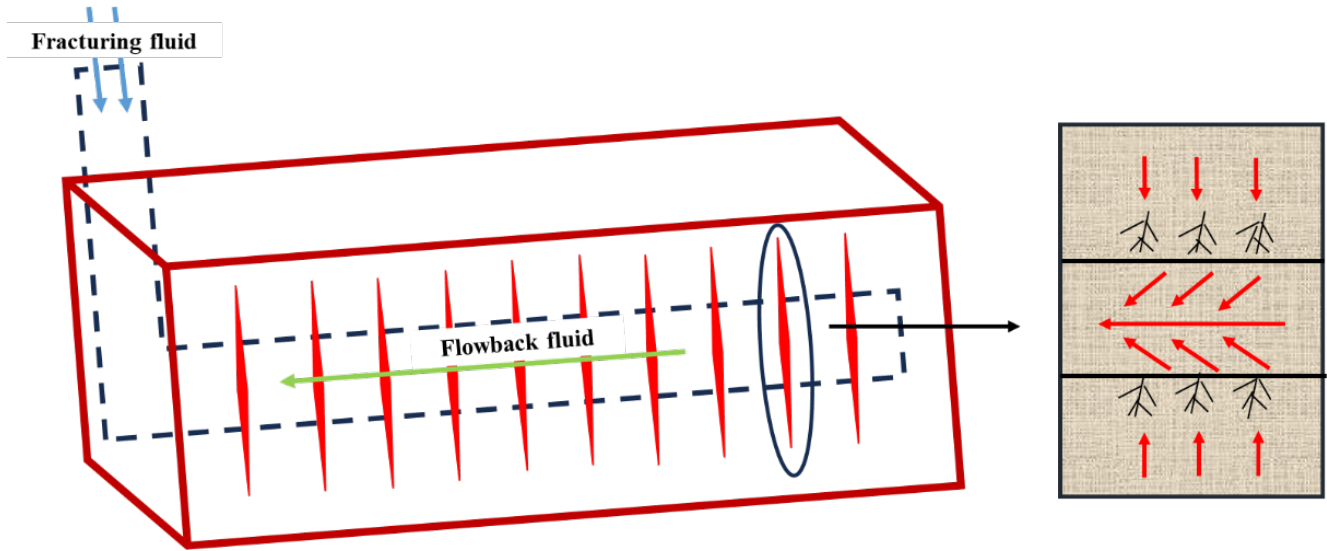
Figure 1. Physical model of a multi-stage fractured horizontal well.
