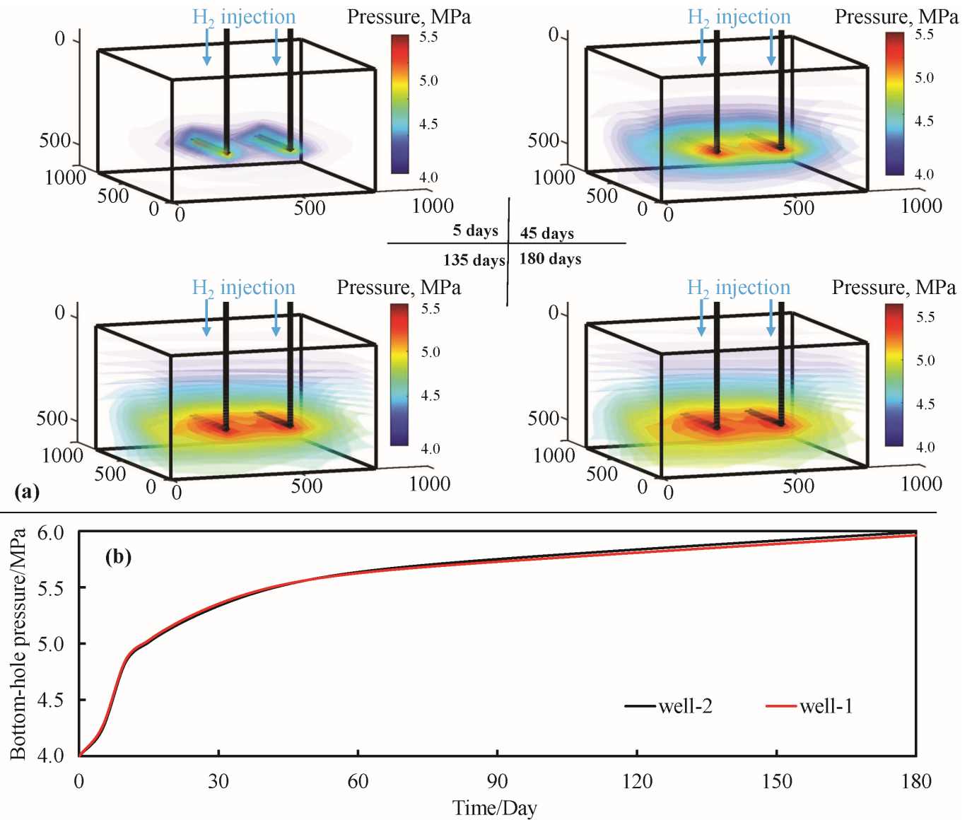
Figure 5. Variation of (a) pore pressure and (b) bottom-hole pressure during H 2 injection over 0.5 year.
