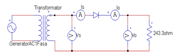
Figure 4. Unfiltered One-Phase half wave uncontrolled rectifier circuit.
