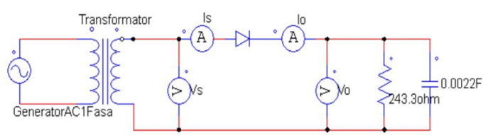
Figure 5. Filtered One-Phase half wave uncontrolled rectifier circuit.
