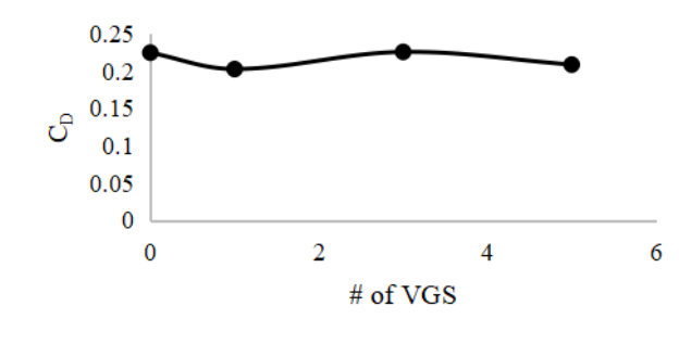
Figure 14. The relationship between C_D and the number of VGs.
