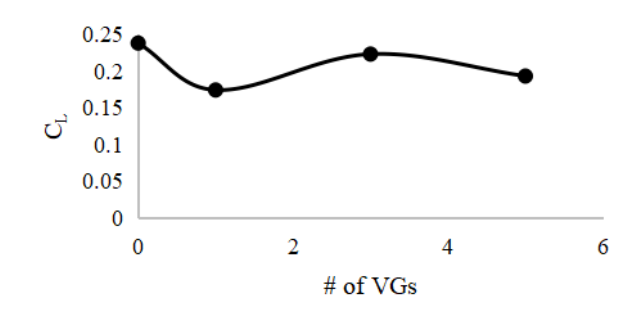
Figure 15. The relationship between C_L and the number of VGs.
