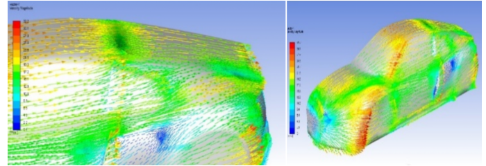
Figure 16. Velocity vector for the vehicle without VGs and Spoiler.
