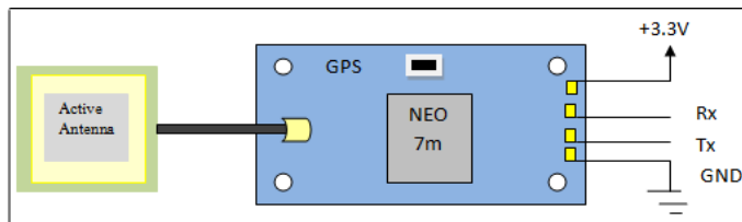
Figure 4. GPS module.
