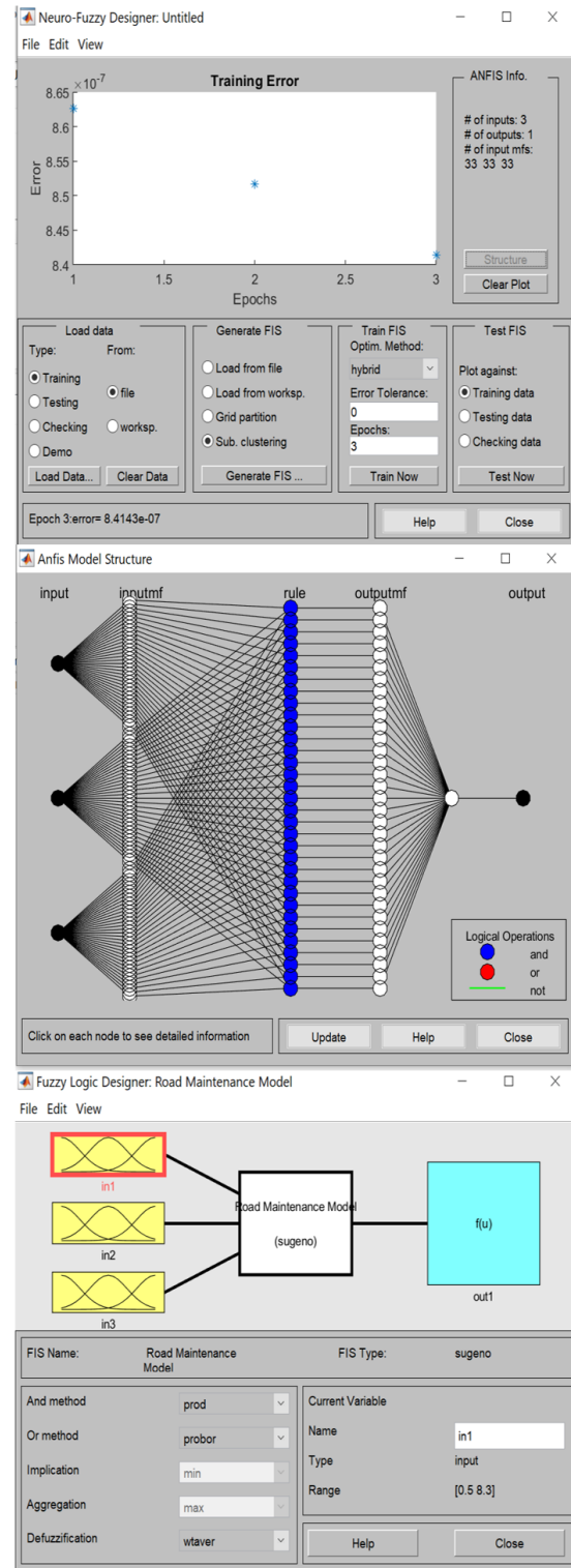
Figure 7. ANFISModel architecture.
