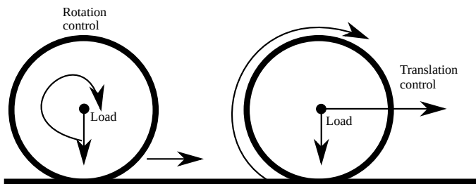
Figure 1. Rotation-controlled and translation-controlled motion of a wheel.
