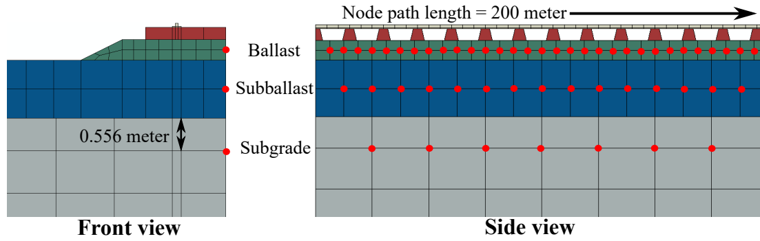
Figure 5. The location of node paths.
