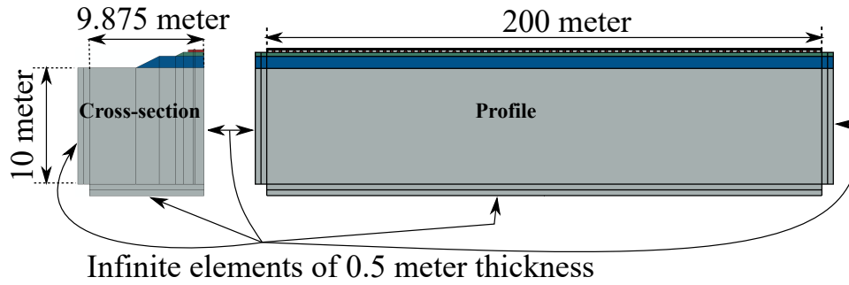
Figure 3. Extents of finite element model in ABAQUS.
