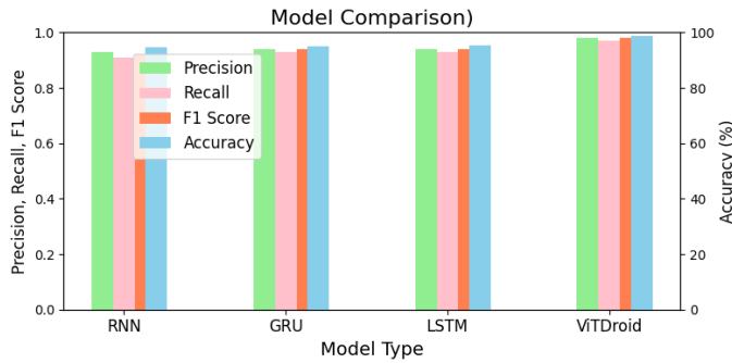
Figure 5. Model comparison: IoT malware detection.
