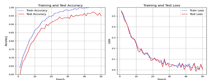
Figure 3. Performance of the LSTM model.
