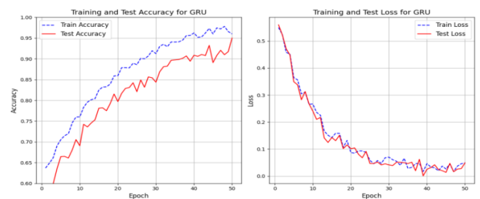
Figure 2. Accuracy of the RNN model.
