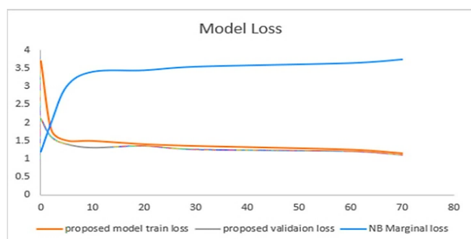
Figure 4. Model loss.
