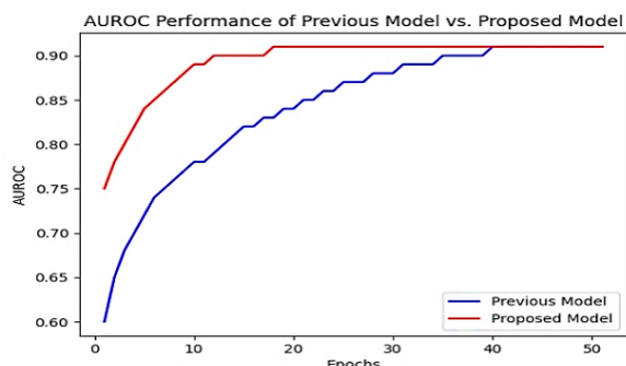
Figure 7. The AUROC performance.
