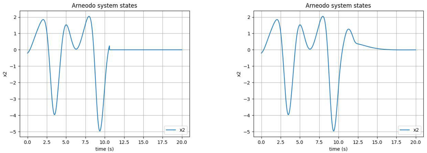
Figure 4. Second state of fractional Arneodo system with control action for time greater than 10 seconds. (Left: \text{sgn}(\cdot) , Right: \tanh(\cdot) ).
