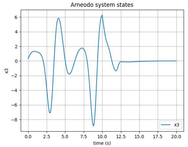
Figure 5. Third state of fractional Arneodo system with control action for time greater than 10 seconds. (Left: \text{sgn}(\cdot) , Right: \tanh(\cdot) ).
