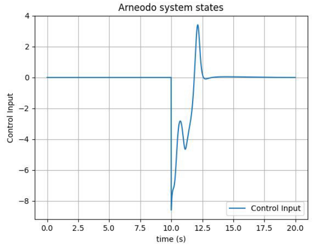
Figure 7. Control Input (Left: \text{sgn}(\cdot) , Right: \tanh(\cdot) ).
