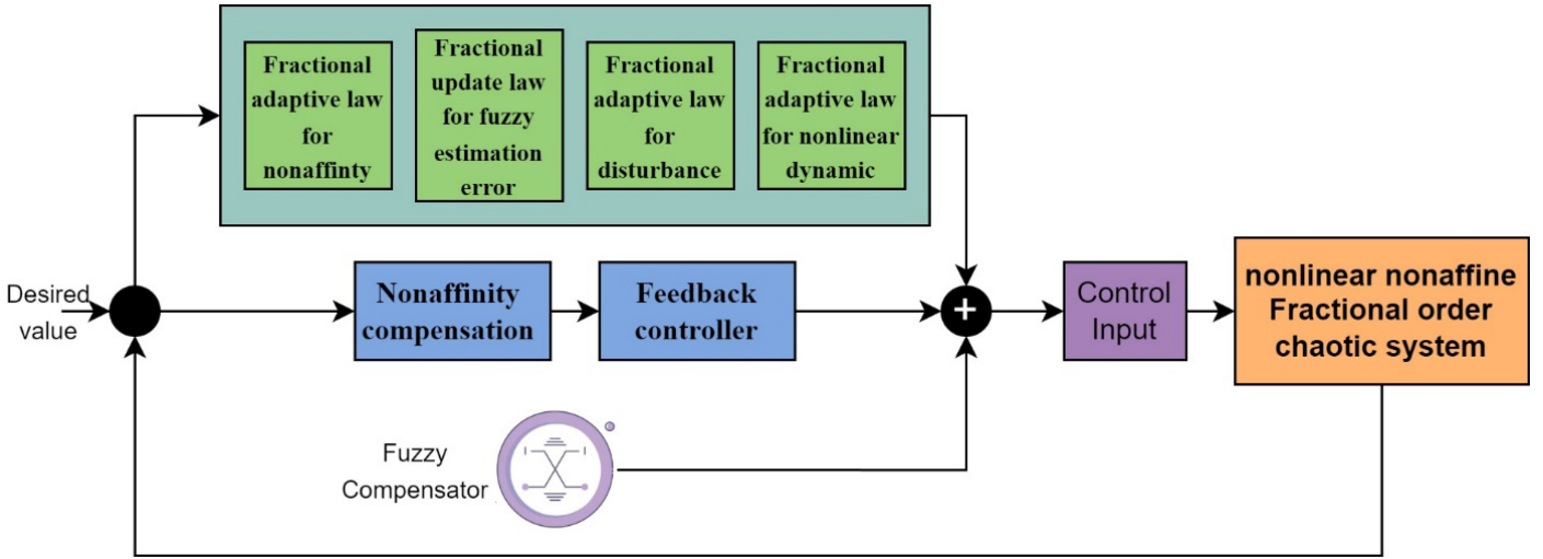
Figure 2. Fractional adaptive fuzzy controller structure.
