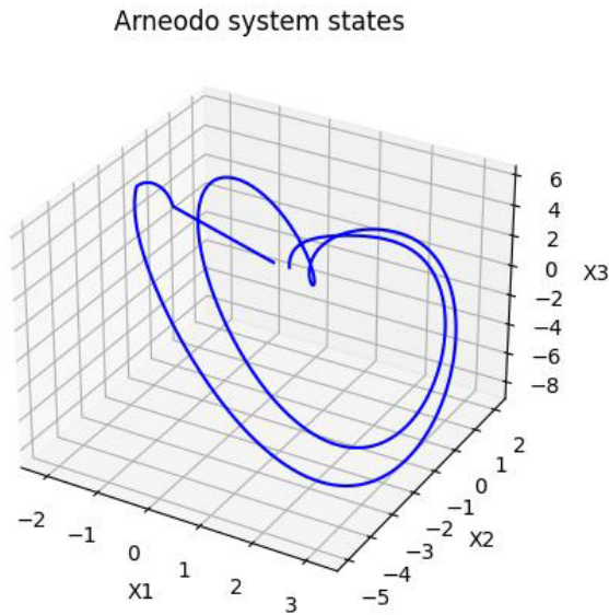
Figure 6. Chaotic attractor of fractional Arneodo system which is stopped its chaotic behaviour in time greater than 10 seconds. (Left: \text{sgn}(\cdot) , Right: \tanh(\cdot) ).
