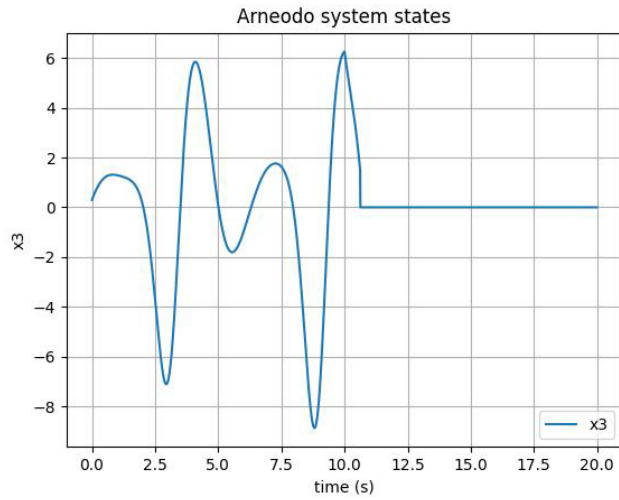
Figure 5. Third state of fractional Arneodo system with control action for time greater than 10 seconds. (Left: \text{sgn}(\cdot) , Right: \tanh(\cdot) ).
