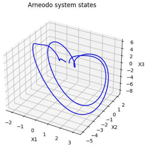
Figure 6. Chaotic attractor of fractional Arneodo system which is stopped its chaotic behaviour in time greater than 10 seconds. (Left: \text{sgn}(\cdot) , Right: \tanh(\cdot) ).
