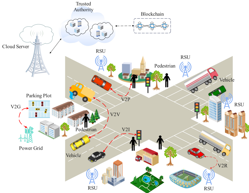
Figure 1. Overview of IoV network architecture.
