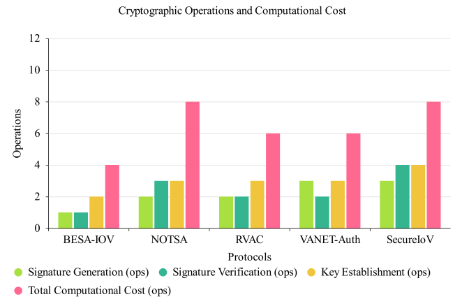
Figure 6. Cryptographic operations and computational cost.
