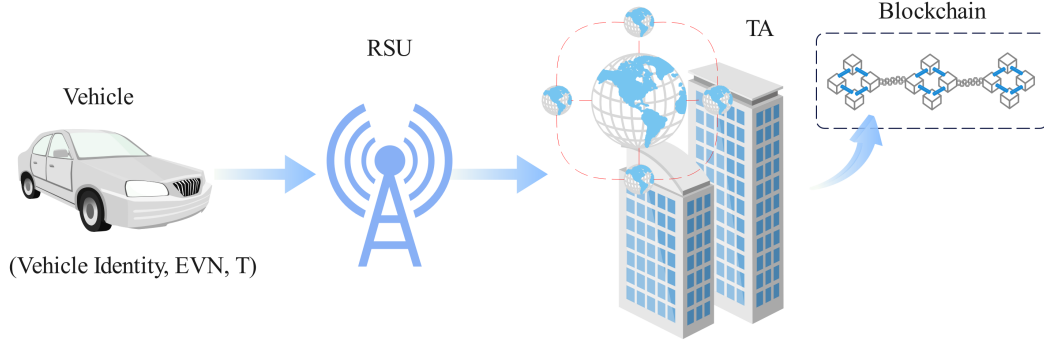
Figure 2. Vehicle registration process in BESA-IOV.
