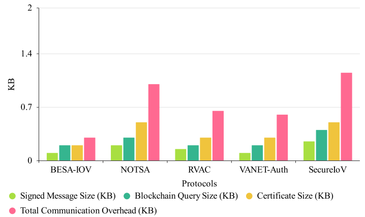
Figure 7. Message size and communication overhead.
