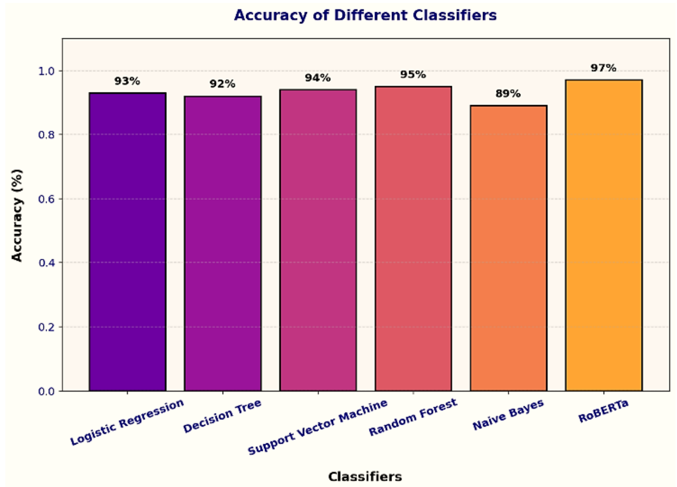
Figure 3. Accuracy comparison of different classifiers.
