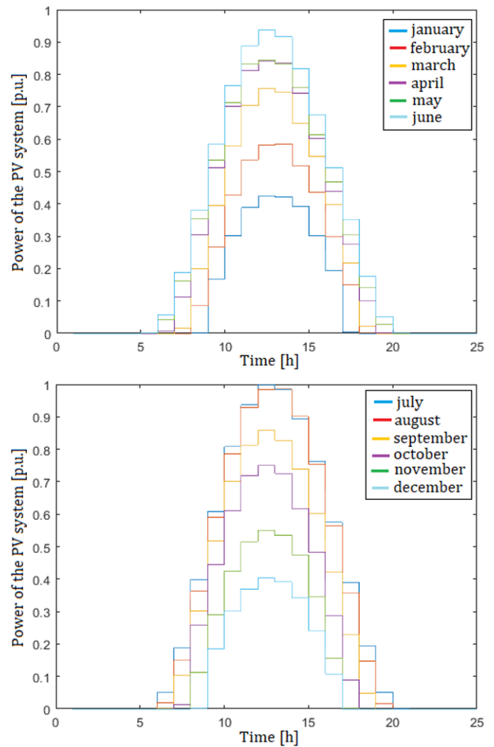
Figure 3. Power generation diagram of the PV system expressed per unit, for the first half of the year (Up) and second half of the year (Down).
