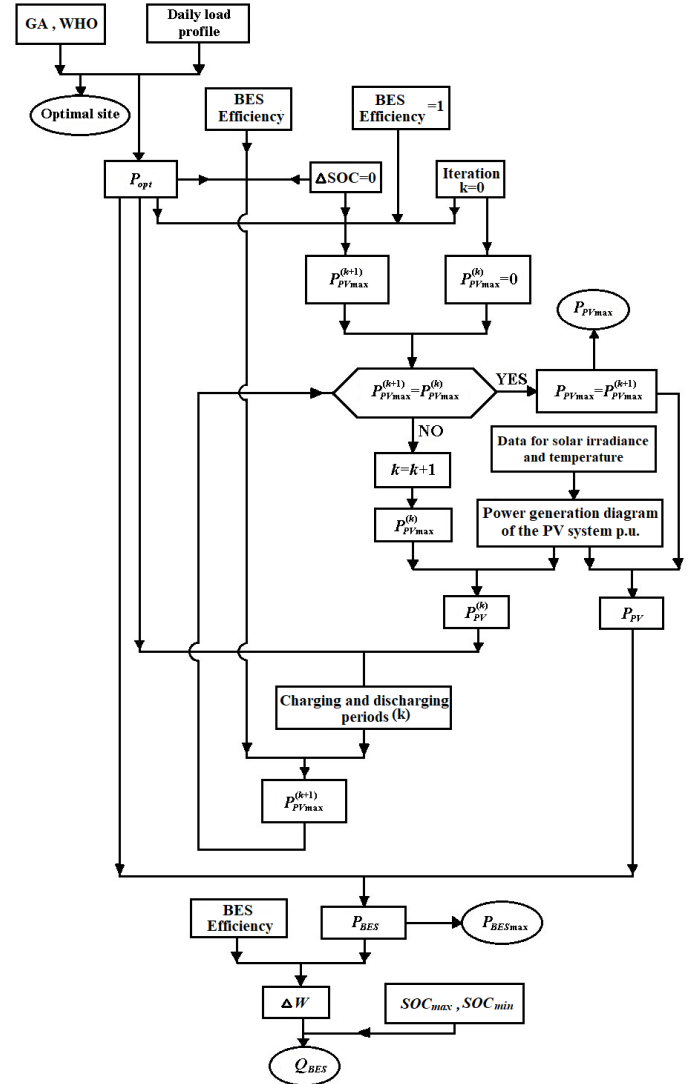
Figure 1. Flowchart of the proposed two-step approach.
