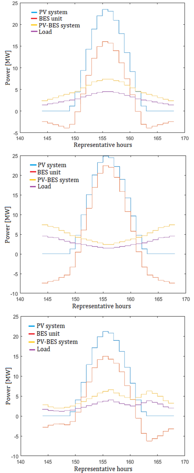
Figure 6. Optimal powers of the PV system, BES unit and the PV-BES system, in July (145-168 representative hour) for the first (Up), second (Middle) and the third load diagram (Down).
