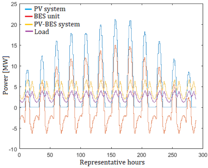
Figure 5. Optimal powers of the PV system, BES unit and PV-BES system, in the one year observation period (288 representative hours) for the third load diagram.
