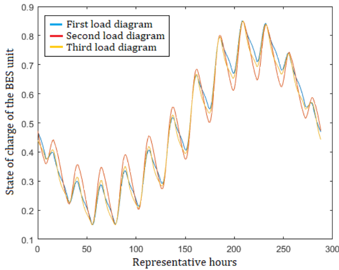
Figure 7. State of charge of the PV-BES system in the one year observation period (288 representative hours) for all three load diagrams.
