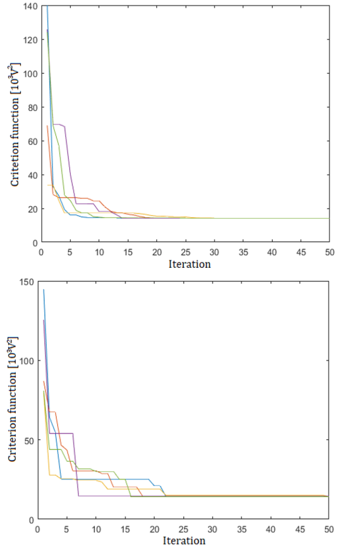
Figure 8. Convergence of the criterion function throughout the iterations obtained using WHO (Up) and GA (Down) for five different runs.
