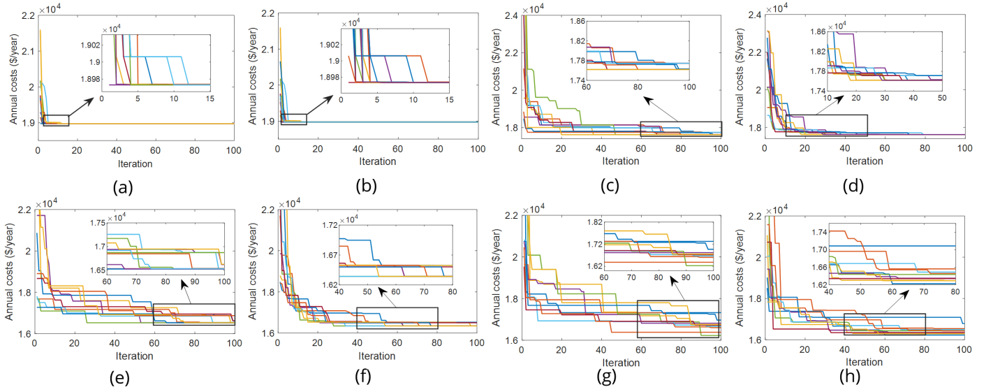
Figure 2. Convergence profiles of the PSO algorithm across different CB configurations. Subfigures (a), (c), (e), and (g) show results obtained using the classic PSO, while (b), (d), (f), and (h) correspond to the Taguchi-based PSO for cases involving 1, 2, 3, and 4 CBs, respectively.
