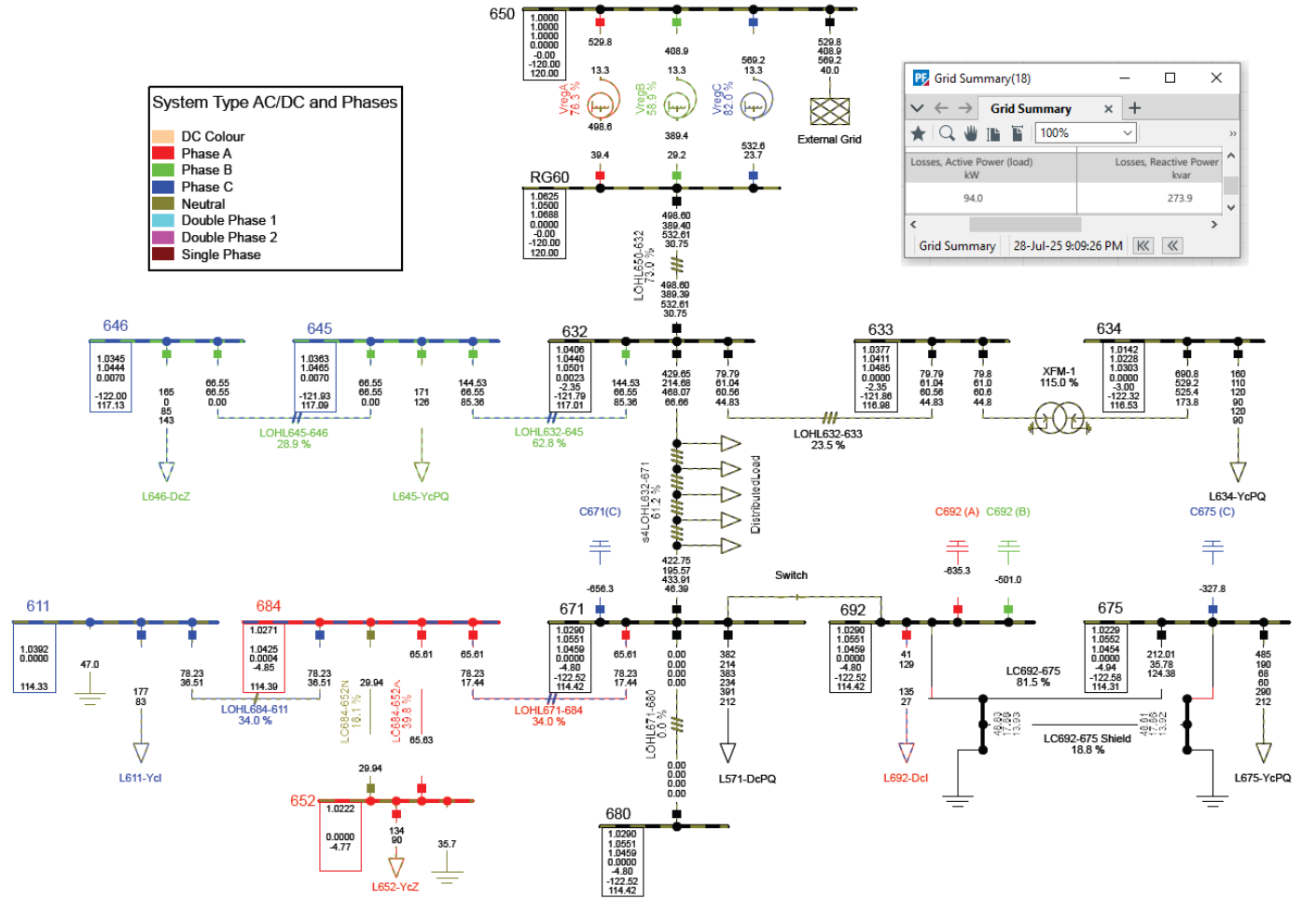
Figure 3. Simulation result obtained using DIgSILENT PowerFactory 2024 for the IEEE 13-bus test system with four installed CBs.
