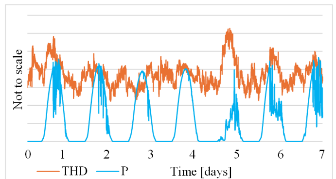
Figure 9. Measured values of the voltage THD factor and PV power plant active power in Period 2.
