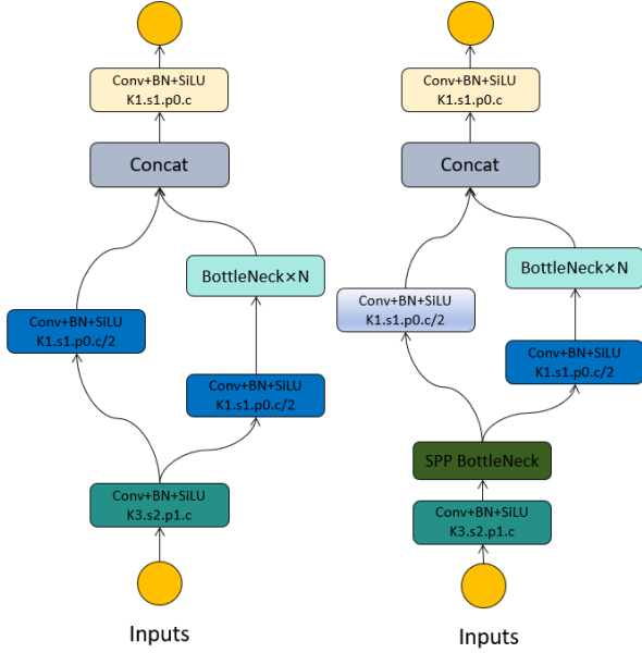
Figure 5. Detailed architectural diagram of the FastDet network.
