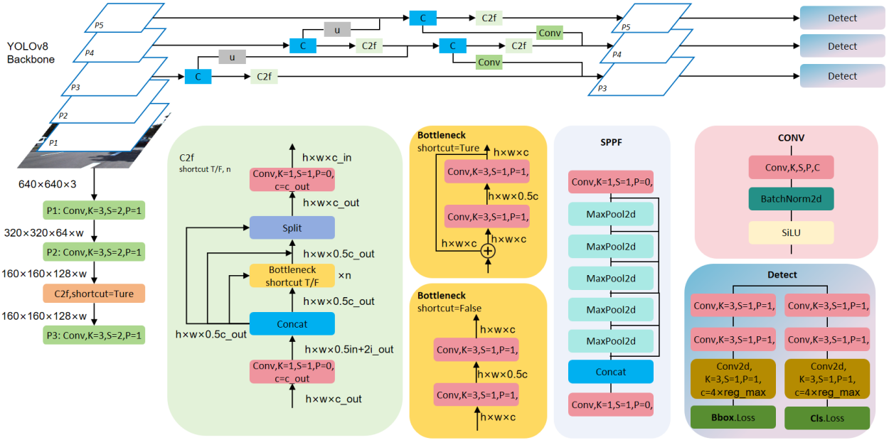
Figure 1. Schematic representation of the YOLOv8 network architecture. The modular design enables adaptation to diverse real-time detection tasks, as demonstrated in smart city applications [32].
