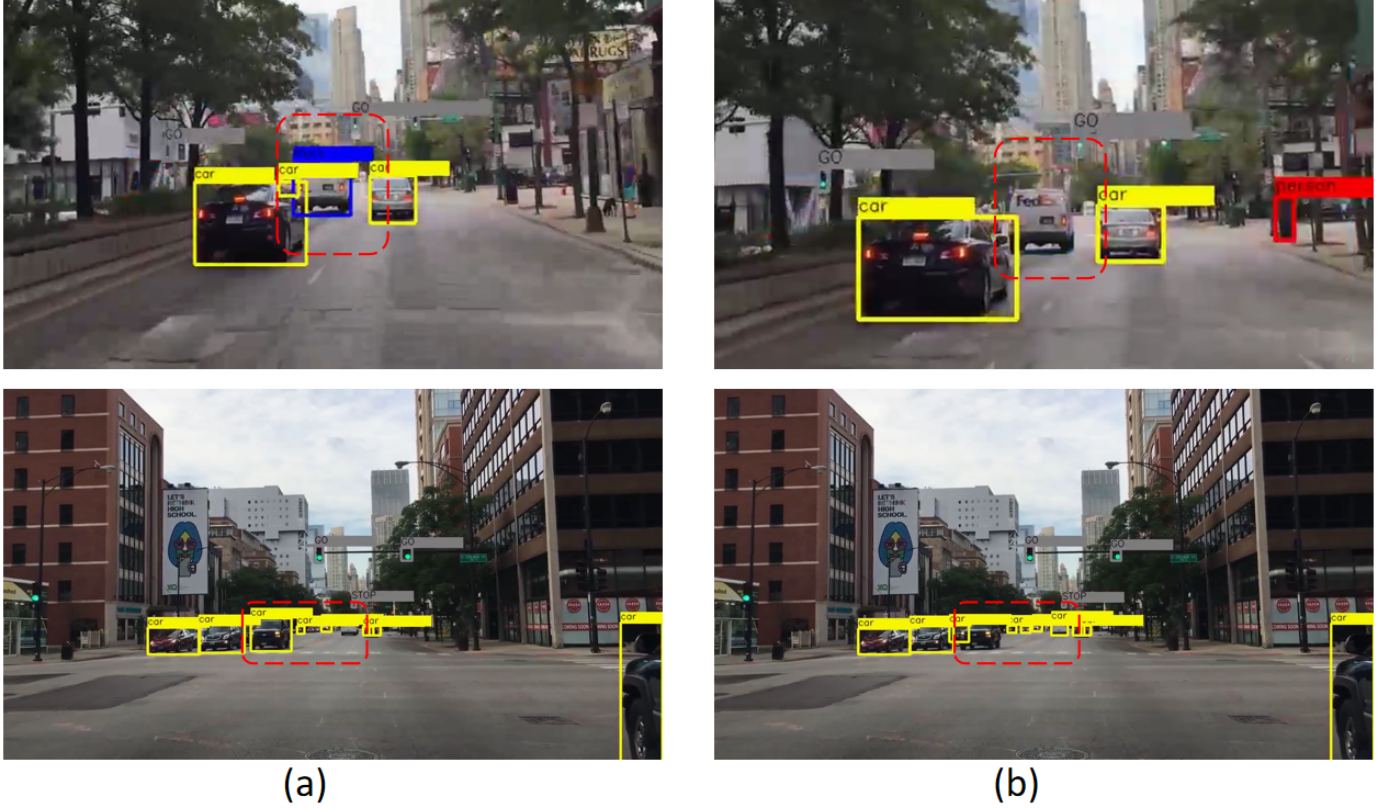
Figure 9. Comprehensive detection analysis. (a) YOLOv8-Lite. (b) YOLOv8.
