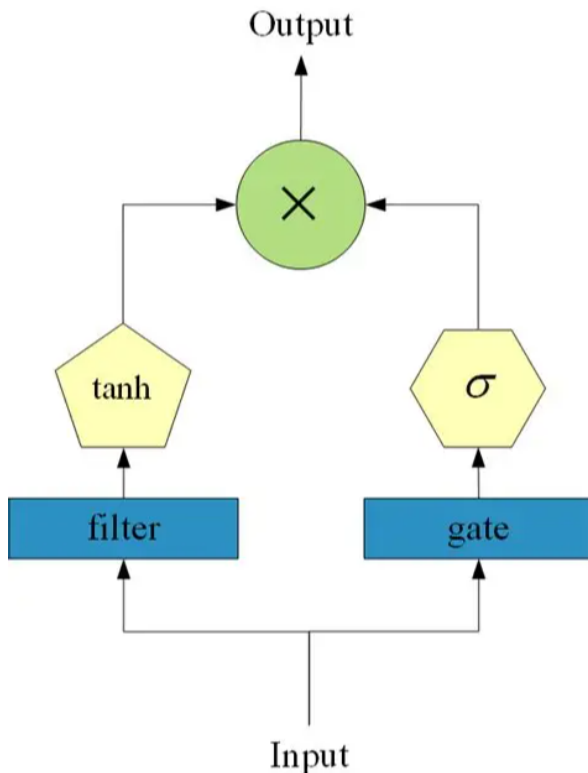
Figure 7. Gated Fusion Unit.
