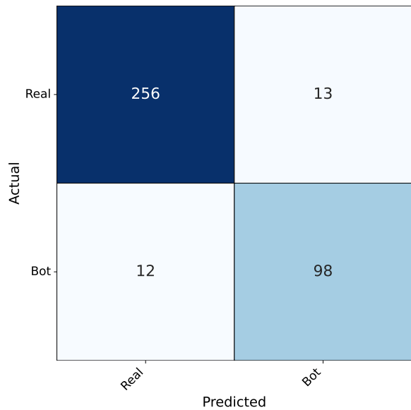
Figure 5. Confusion matrix illustrating the proposed model’s performance.
