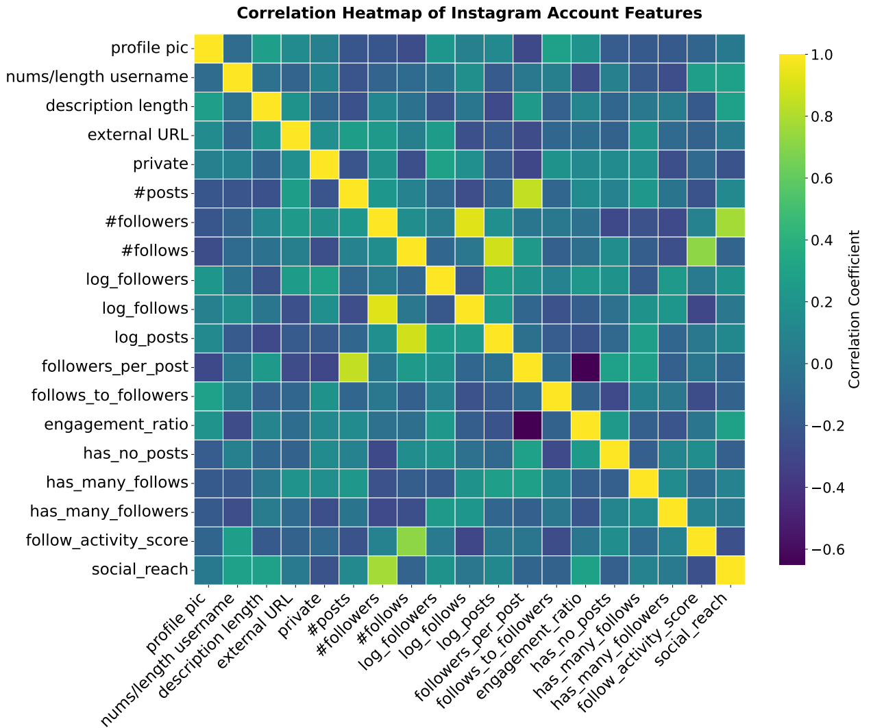
Figure 4. Correlation heatmap visualizing the relationships between features.
