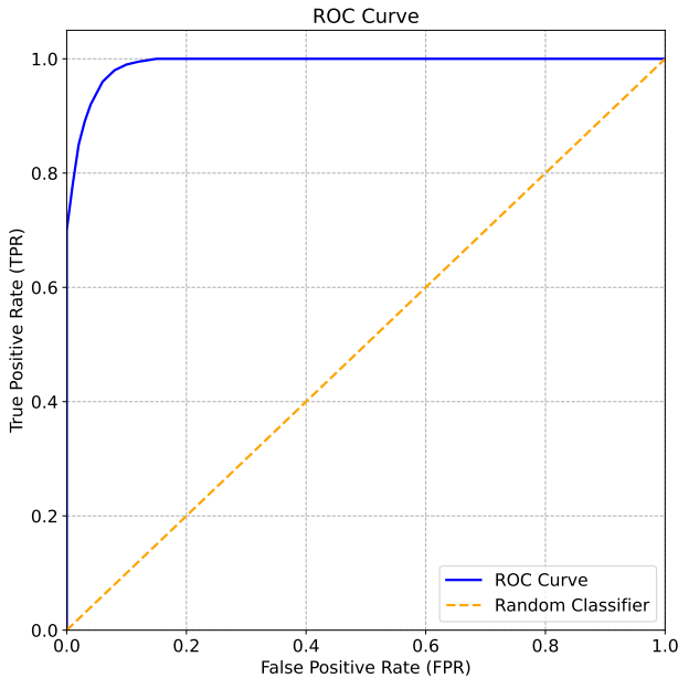
Figure 6. Receiver Operating Characteristic (ROC) curve for the proposed model for real and bot classification.
