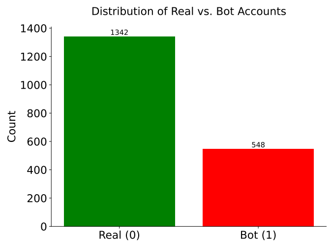
Figure 2. Distribution of samples across real and bot classes.
