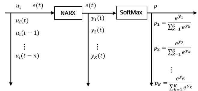
Figure 2. The workflow of the NARX-SoftMax model. The input layer consists of current and past input values u_i(t), u_i(t-1), \dots, u_i(t-n) along with an error term \xi(t) . These inputs are processed by the NARX model to produce an intermediate output y_j(t) , which is converted into probabilities p_j for each class j by the SoftMax classifier.
