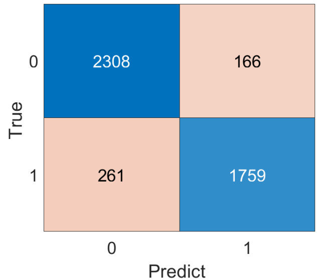
Figure 9. Confusion matrix of the NARX-SR predictions (test set).
