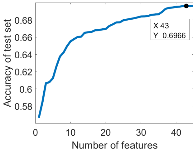
Figure 11. The Accuracy plot of NARX-SR (test set).
