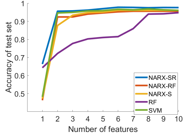
Figure 7. A comparison of different methods in feature selection (test set).
