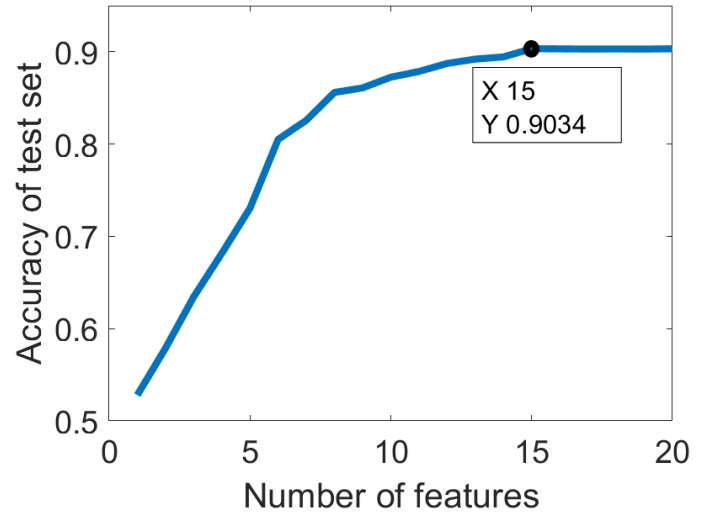
Figure 8. Accuracy plot of NARX-SR (test set).
