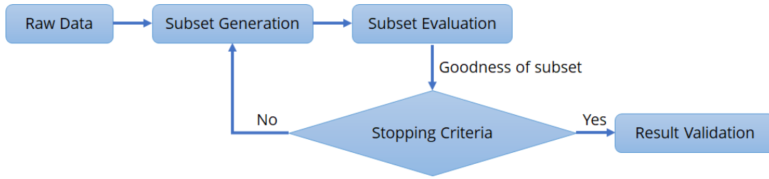
Figure 1. Forward orthogonal search and selection process.
