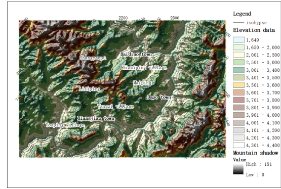
Figure 5. Topographic map of the study area.
