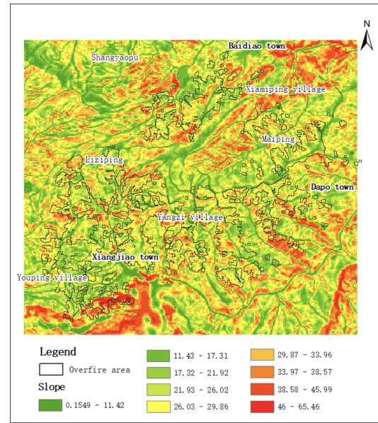
Figure 6. Slope map of fire area.
