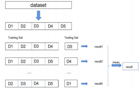
Figure 2. 5-fold cross-validation
