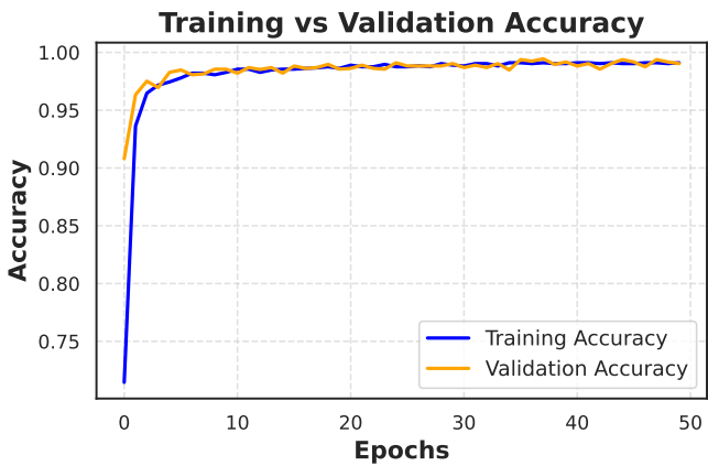
Figure 5. Training and validation accuracy curves for the GCViT model over 50 epochs.
