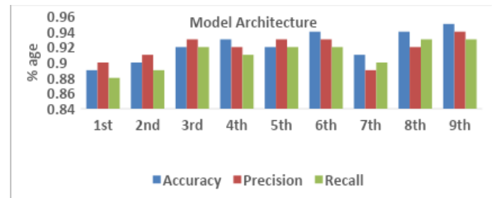
Figure 5. Performance comparison: ReLU activation.
