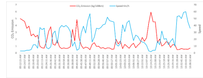
Figure 7. Carbon dioxide ( CO_2 ) Emission and Speed.
