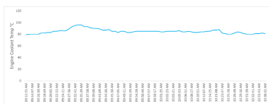
Figure 14. Coolant Temperature of Vehicle.
