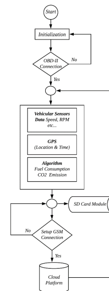
Figure 2. The Cyber-Physical system flowchart for vehicles.
