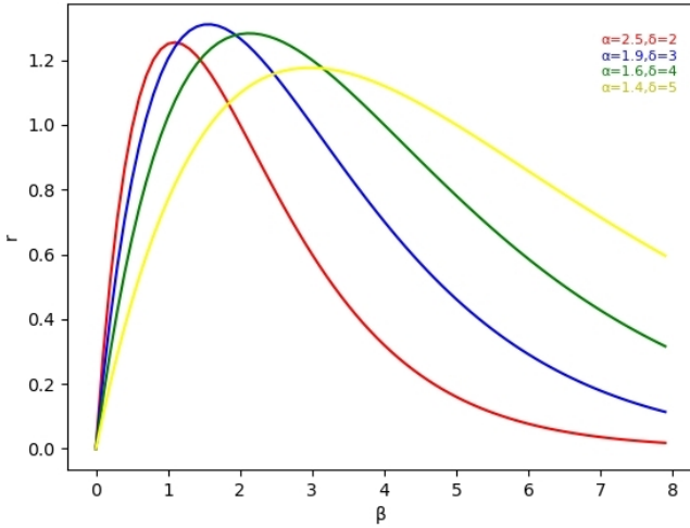
Figure 2. Effect of hyperparameters \alpha and \delta on the mapping between outlier \beta and gradient gain r .
