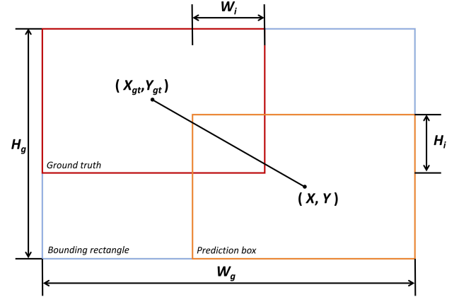
Figure 1. Example of BBR loss.
