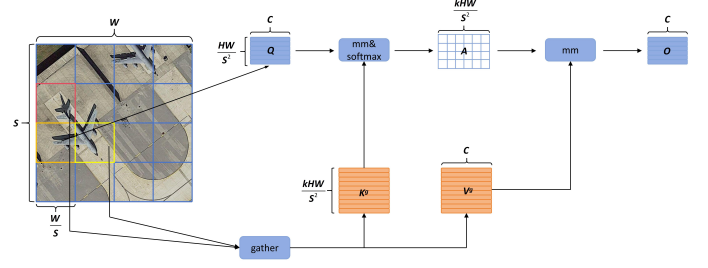
Figure 4. Schematic diagram of BRA principle.
