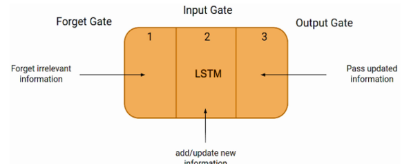
Figure 3. LSTM Architecture [4].
