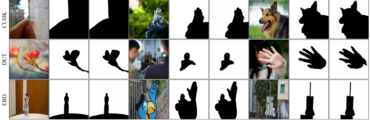
Figure 2. Qualitative results of SemanticBlur on representative samples from the CUHK-TE, DUT, and EBD datasets. For each row, from left to right: input image, ground truth annotation, and the predicted defocus blur map. The proposed method effectively localizes defocused regions while maintaining sharp boundary details across diverse photographic scenarios.
