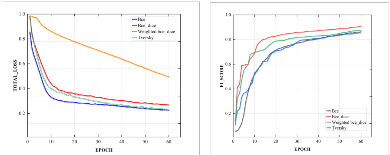
Figure 11. The variation of model loss function with epochs: (a) Total loss function; (b) F1-score function.
