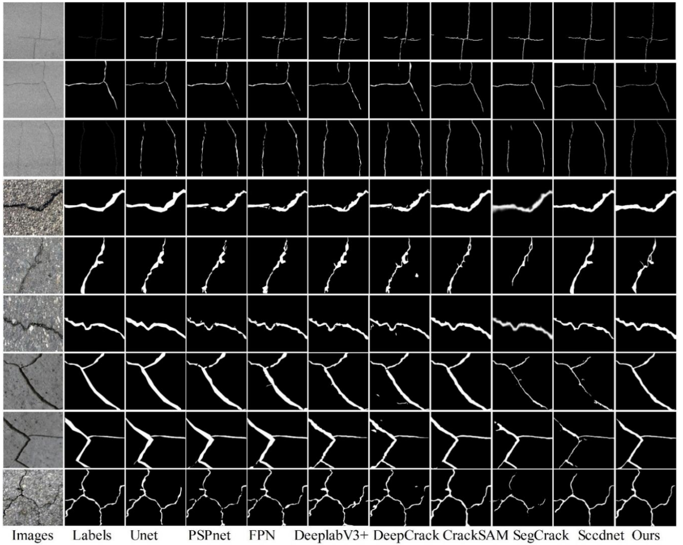
Figure 13. The segmentation results of the proposed model and the comparative model on three datasets.
