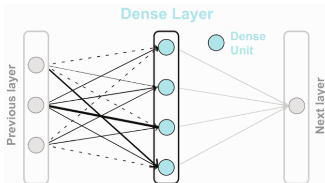
Figure 4. Visualization of the Additional Dense Layer in the Neural Network.
