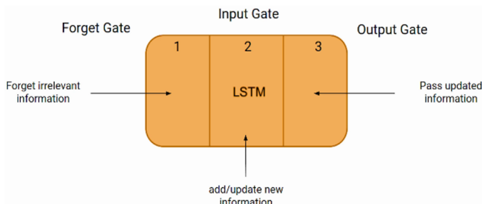
Figure 3. LSTM Architecture [4].
