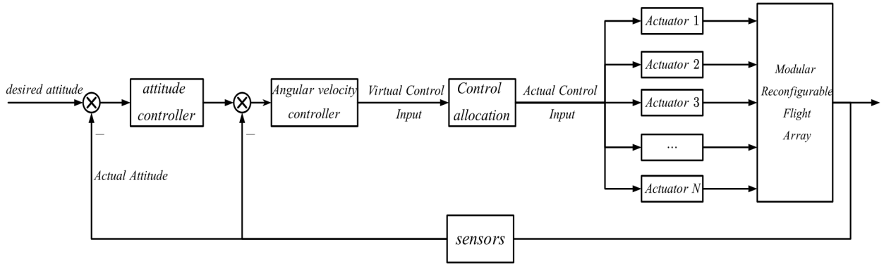
Figure 5. Reconfigurable flight array control diagram.
