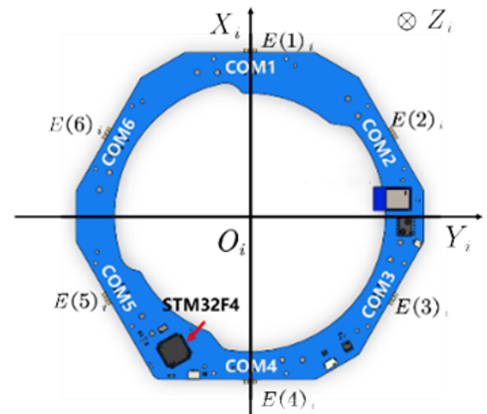
Figure 3. Communication module circuit board.
