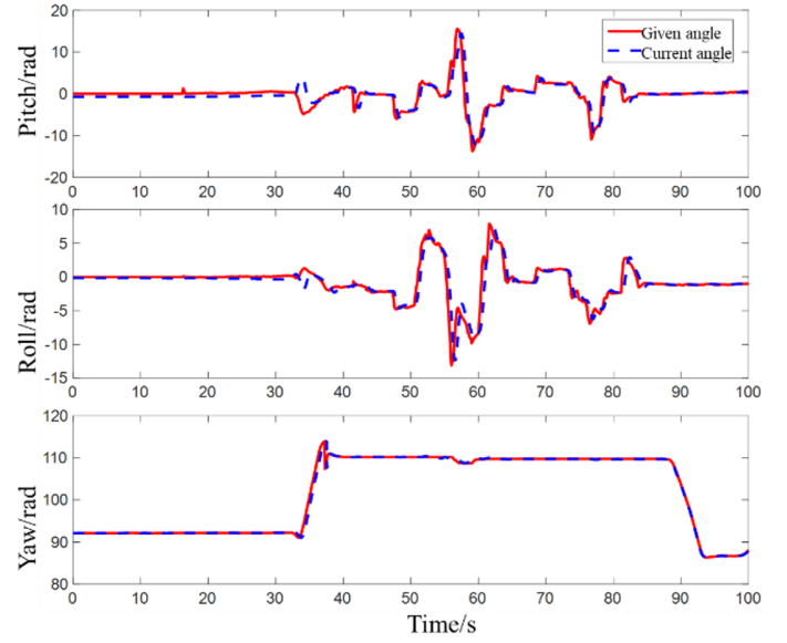
Figure 8. Attitude tracking curves of reconfigurable flight array.
