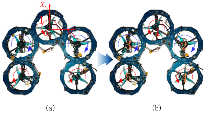
Figure 6. Five-module reconfigurable flight array.
