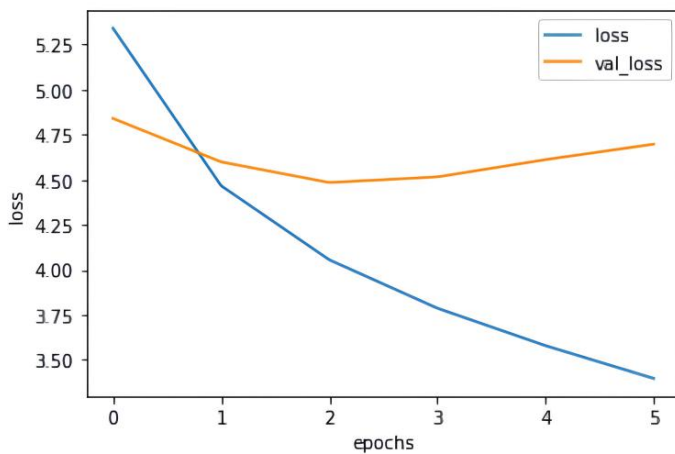
Figure 10. Existing Train-Val graph.
