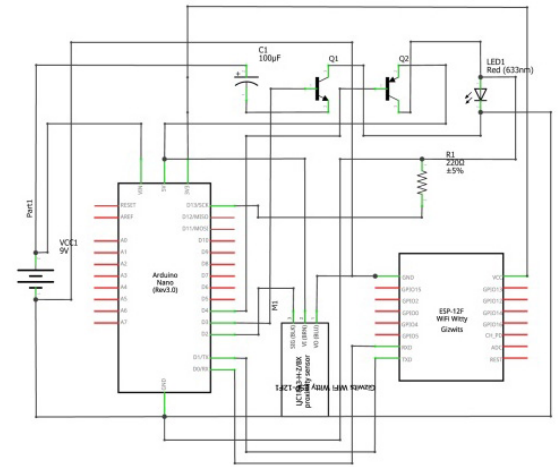
Figure 2. Mine detection devices circuit diagram.
