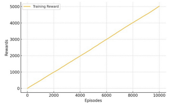
Figure 7. Training rewards.
