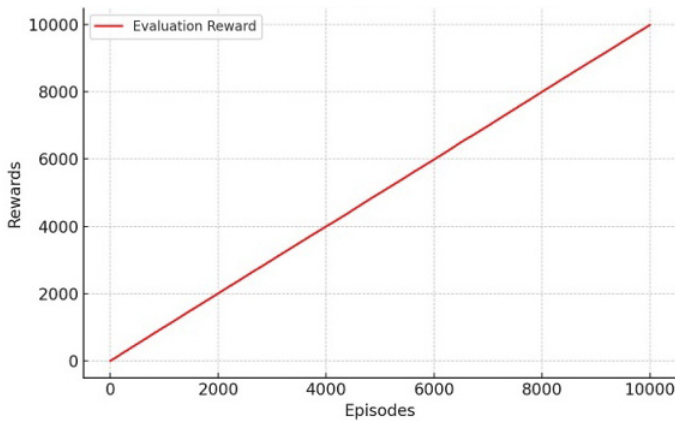
Figure 6. Evaluation rewards.
