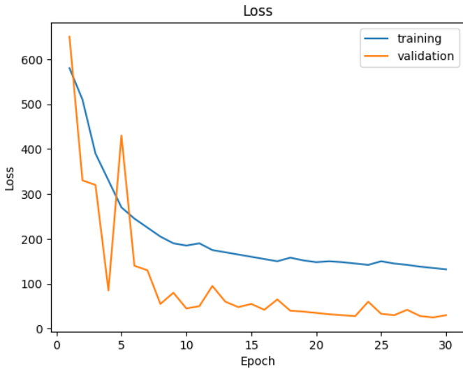
Figure 20. Validation and training loss of moderate model from 1 to 30 epochs.
