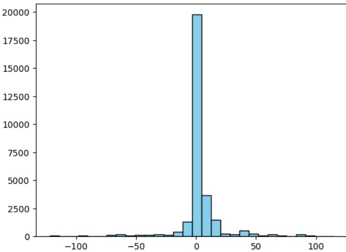
Figure 1. Dataset Distribution.
