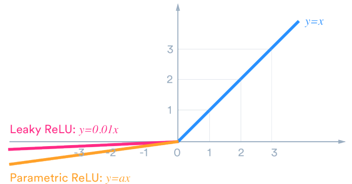
Figure 9. Leaky ReLU.
