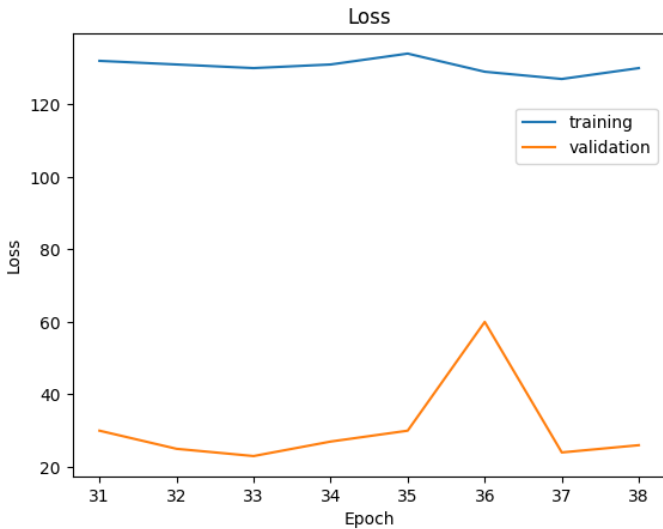
Figure 21. Validation and training loss of moderate model from 31 to 38 epochs.
