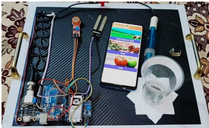
Figure 6. Complete project setup featuring pH, moisture, and ethanol sensors integrated with Arduino UNO and NodeMCU.
