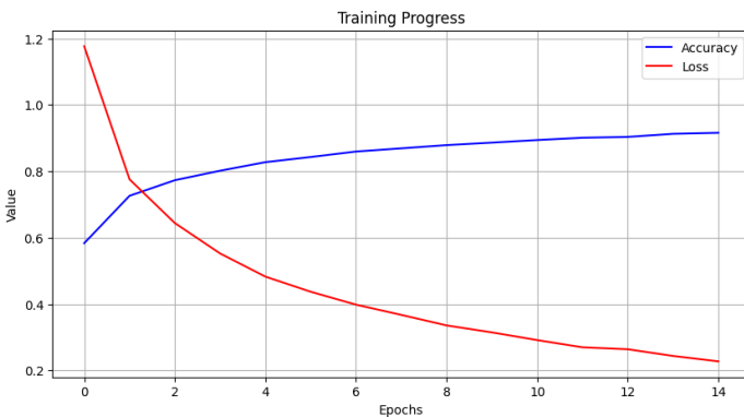
Figure 6. Training accuracy and loss.
