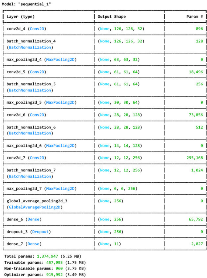
Figure 3. Model summary.
