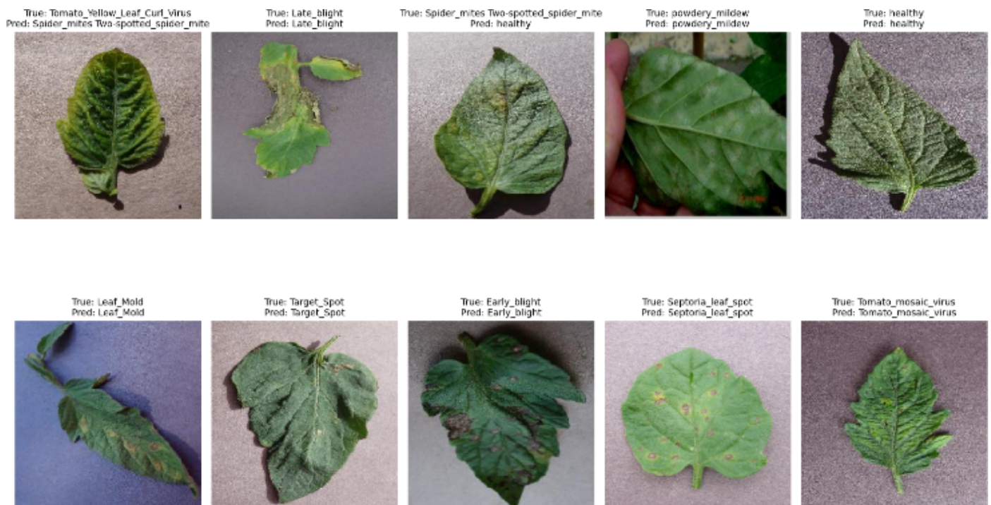
Figure 8. Classified images.
