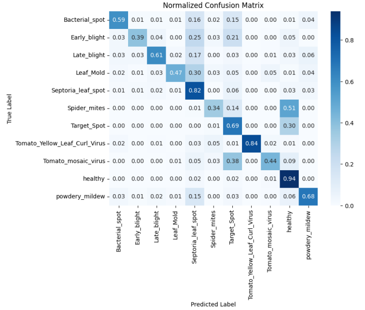
Figure 7. Confusion matrix.
