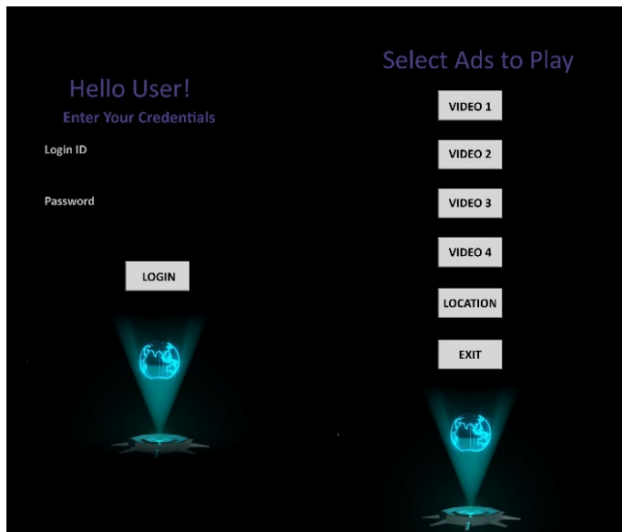
Figure 4. Android Application.
