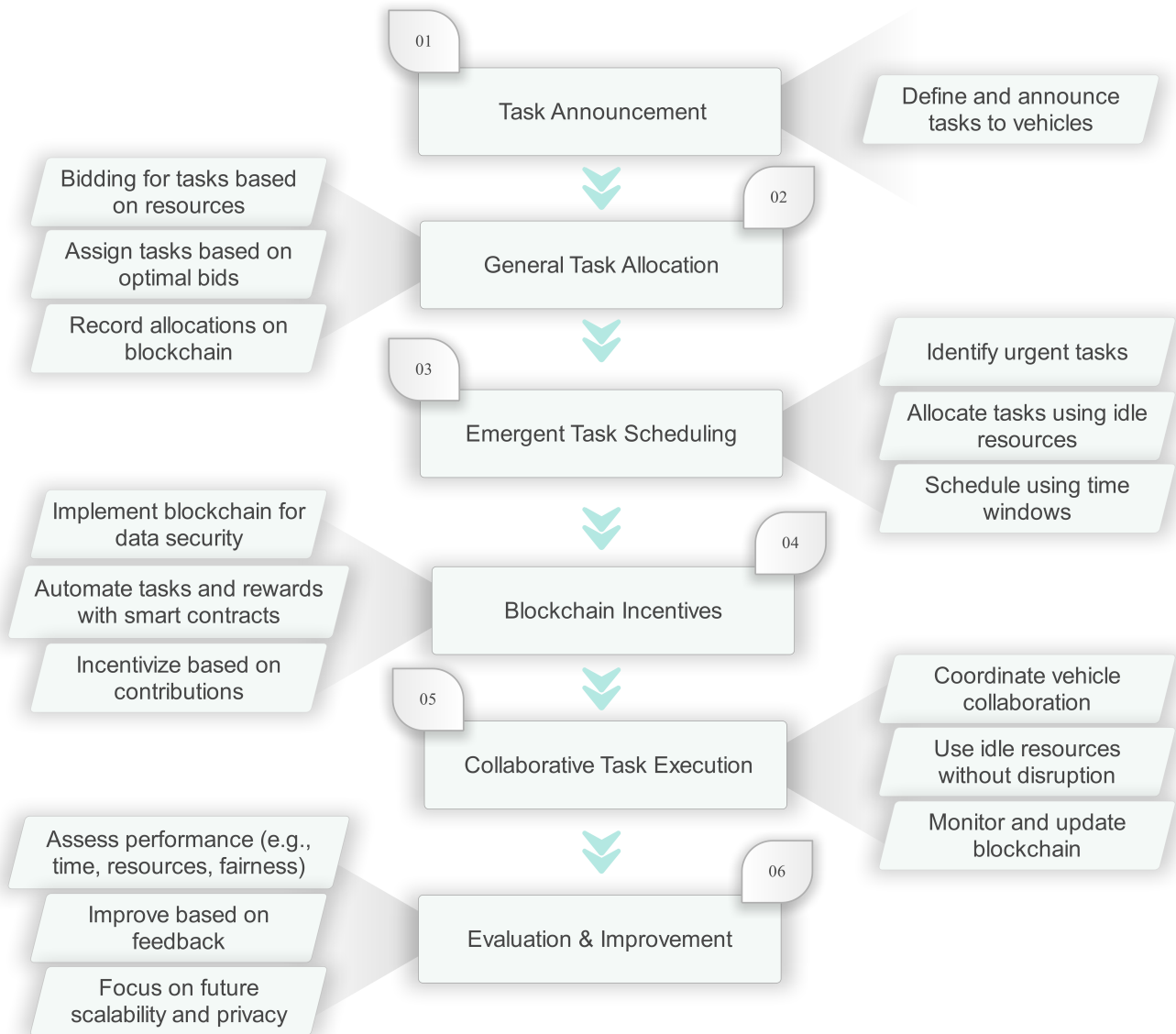
Figure 2. Flowdiagram of proposed blockchain-based task allocation and reward distribution in IoV.
