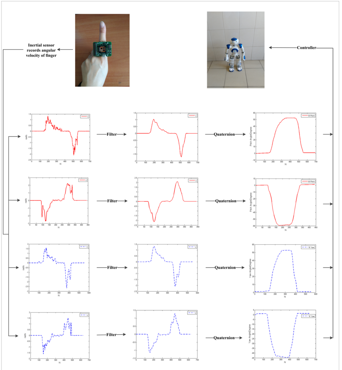
Figure 4. The diagram of the algorithm.
