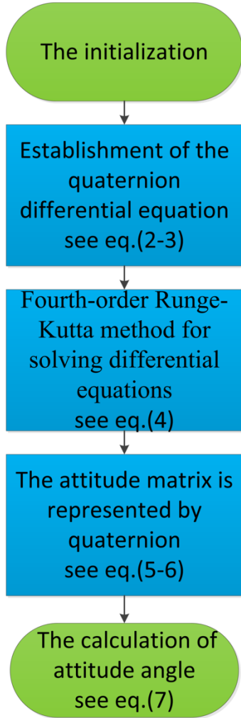
Figure 1. Flow diagram of quaternions method.
