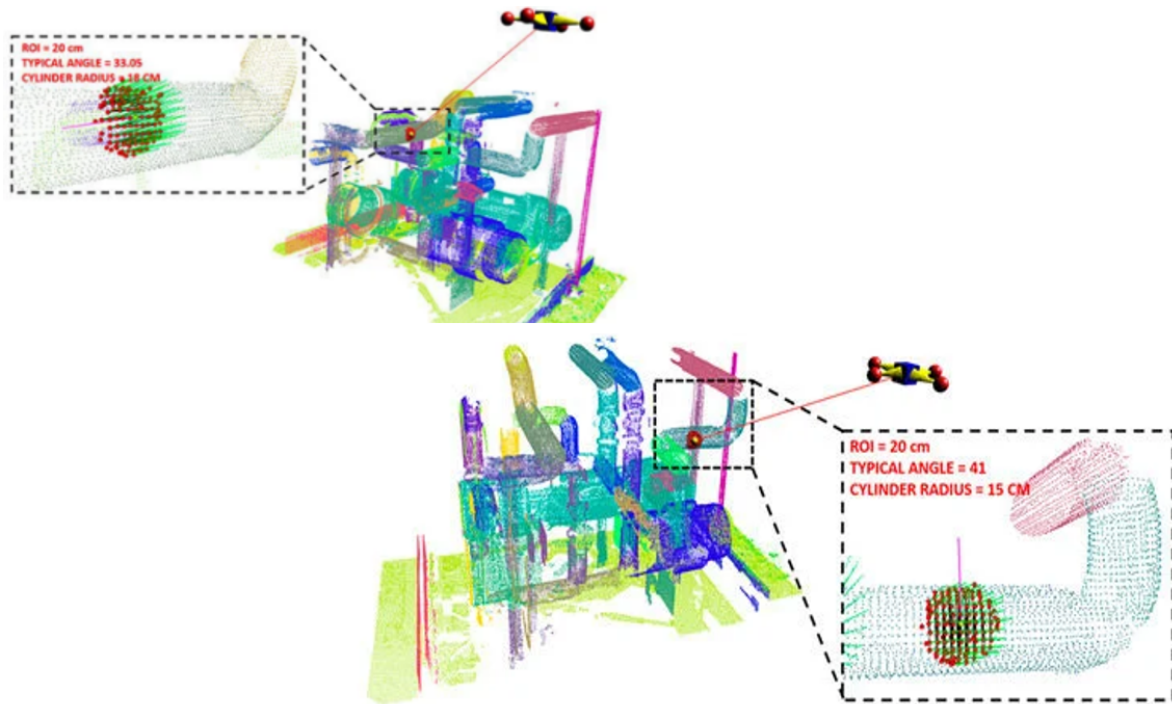
Figure 3. Indoor mapping and combined sensor.
