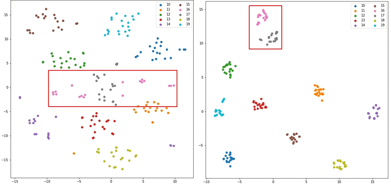
Figure 3. UCF101 partial category feature clustering visualization.
