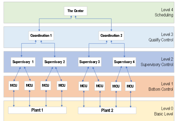
Figure 4. Conventional hierarchical manufacturing control operation [32].
