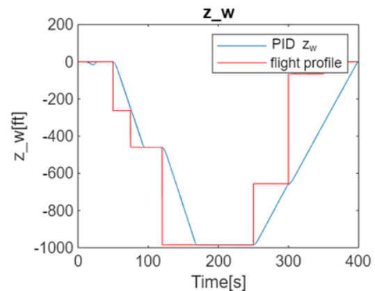
Figure 9. output z_w low speed controller.
