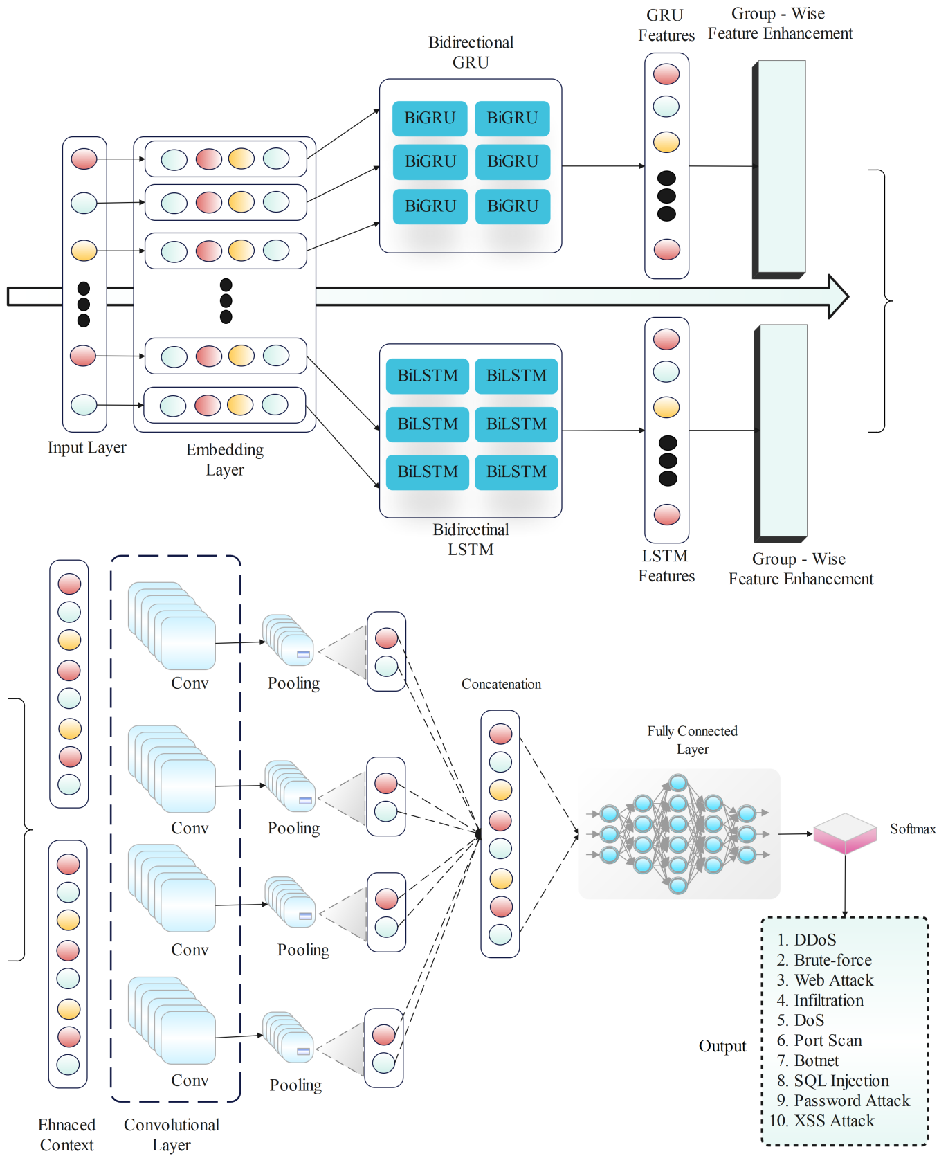
Figure 3. Proposed architecture.
