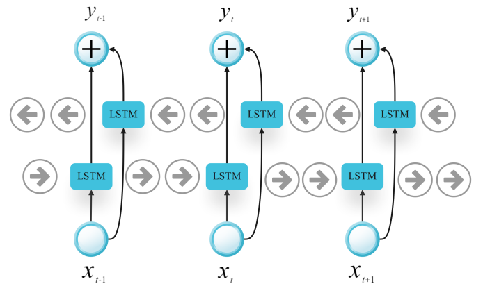
Figure 1. BiLSTM.
