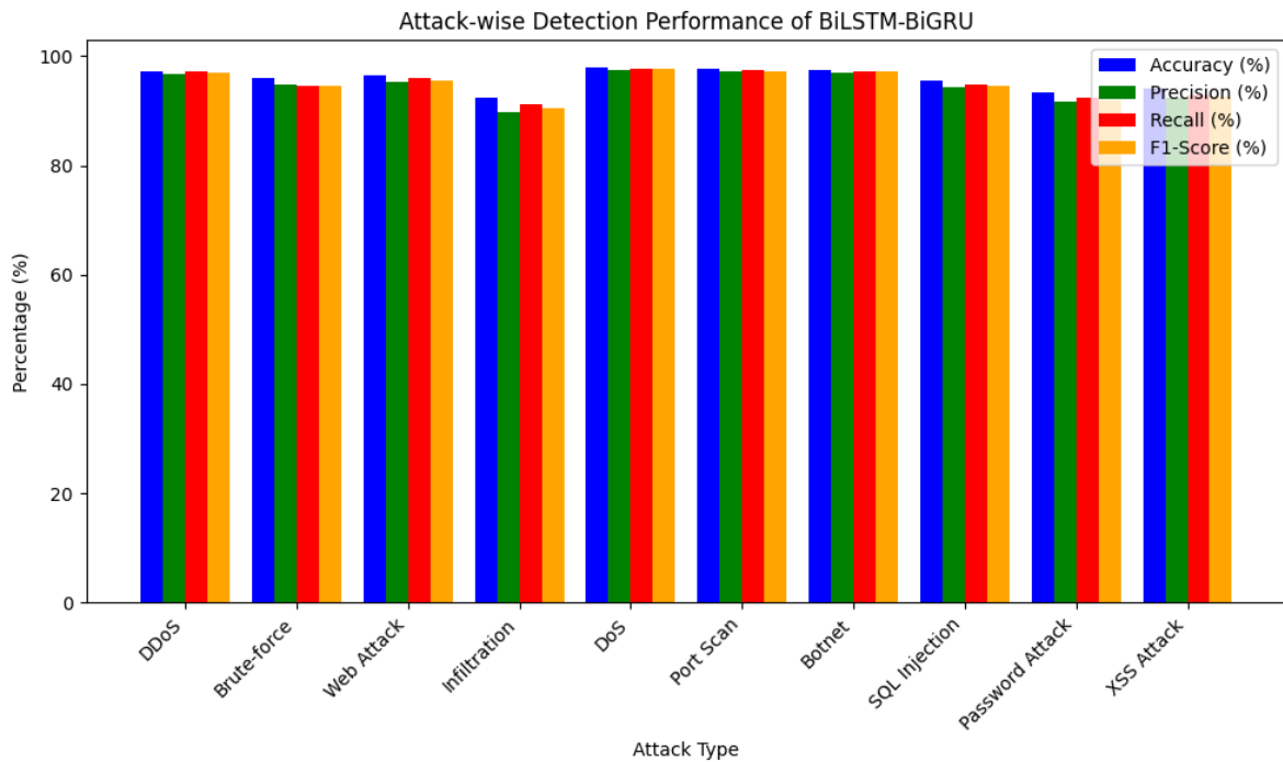
Figure 7. Attack Wise Metrics.
